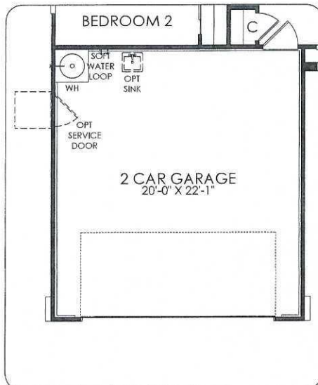
70970 - Garage Extension 2'
