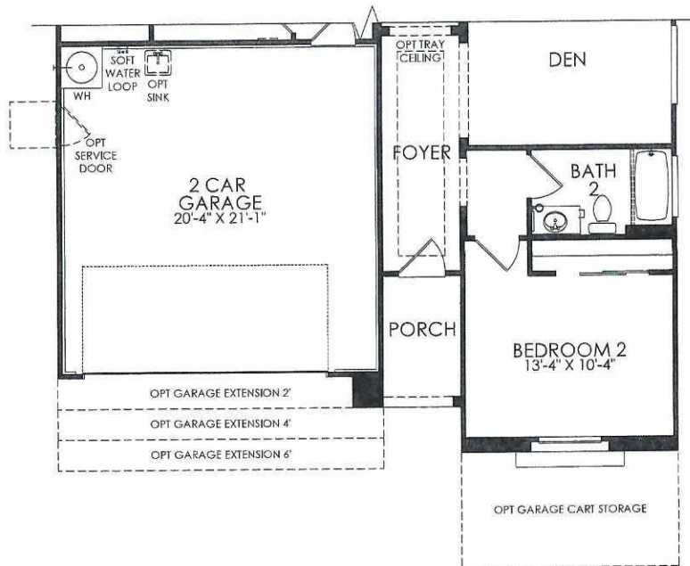
Floor Plan Elevation 'B'
