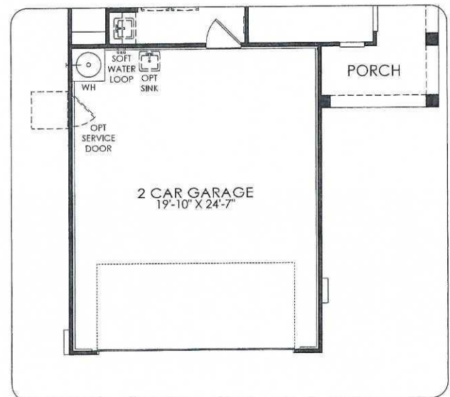
70971 - Garage Extension 4'
