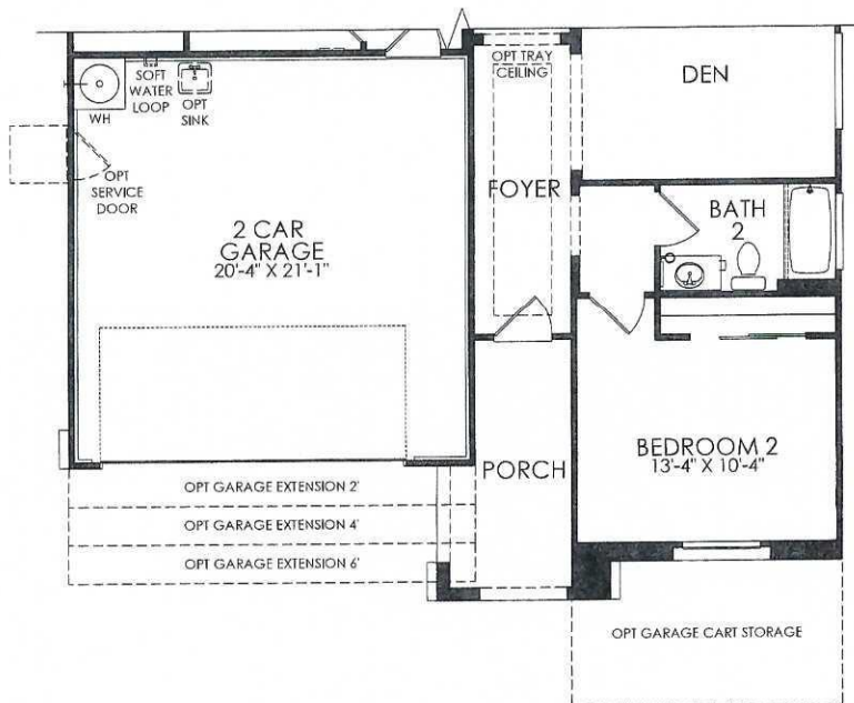
Floor Plan Elevation 'C'
